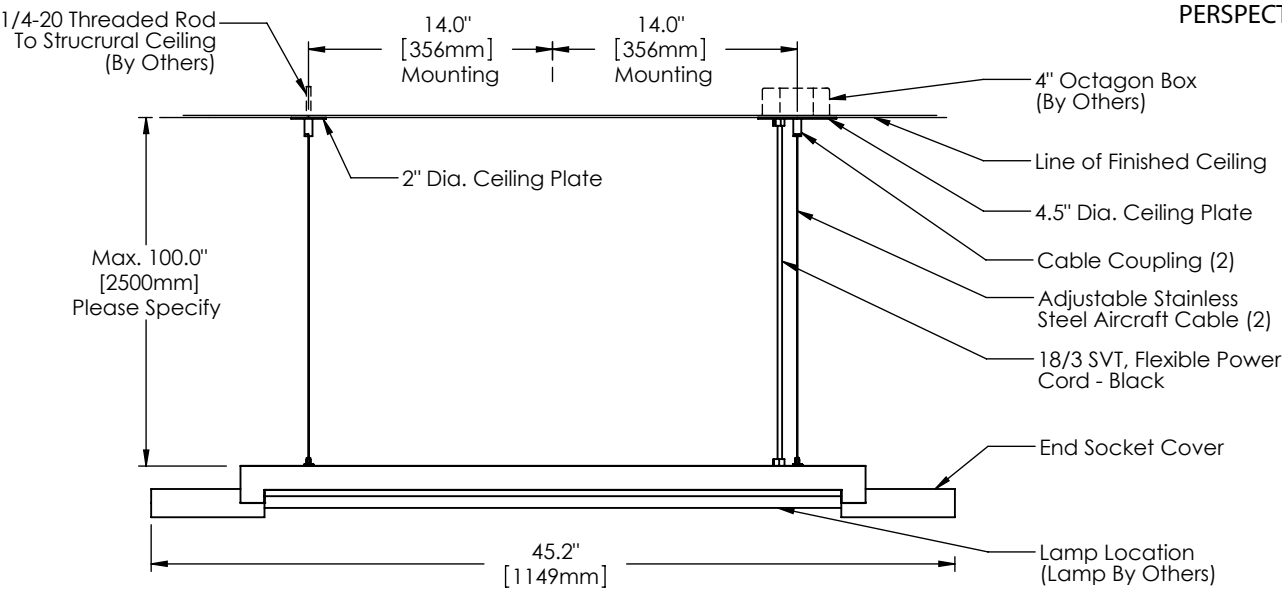
PERSPECTIVE VIEW
