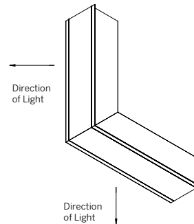
Mitered + Welded Housing Mitered + Butted Lens
