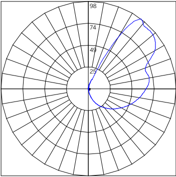
ISOILLUMINANCE DIAGRAM - LOW POWER 3500K WG-60SCFW-...-L-92-35-...-W 1
