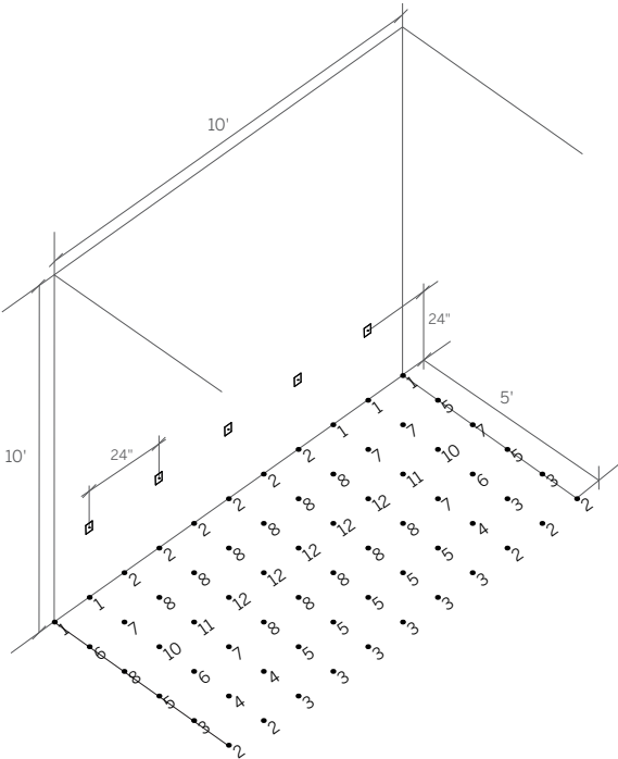
ISOILLUMINANCE DIAGRAM - LOW POWER 3500K WG-60SCFW-...-L-92-35-...-W 1
