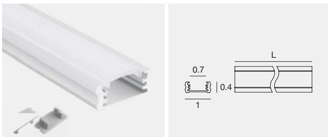
Ozner_25/10 | Low surface profile
