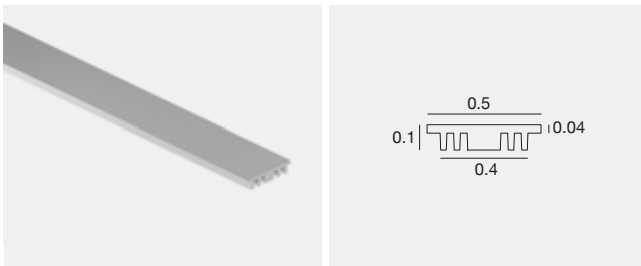
Svik_00/00 | Heat sink
