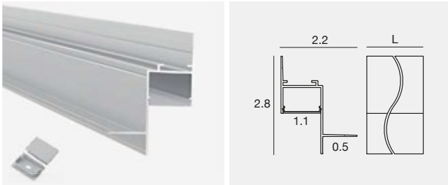
Rialt_55/70 | Integrated side profile
