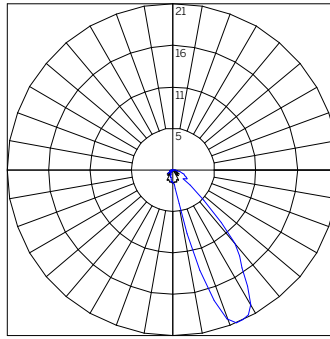
Beam Angle (0-180) = Asymmetric Beam Angle (90-270) = Asymmetric
