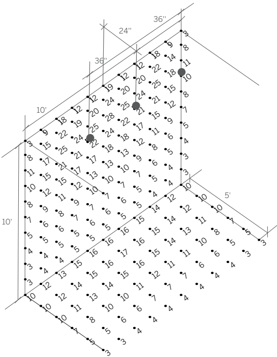
ISOILLUMINANCE DIAGRAM - HIGH POWER 3500K WG-60RGDL-...-H-935-...-RSRWW-RSC-RWW-W-W 1
