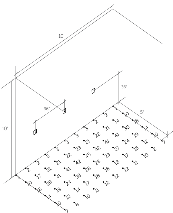
ISOILLUMINANCE DIAGRAM - HIGH POWER 3500K WG-100SCFW-...-H-92-35-...-W 1
