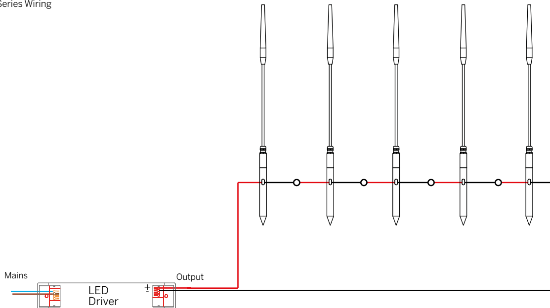
Series Wiring
