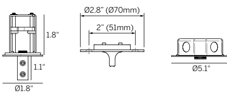
2" dia
