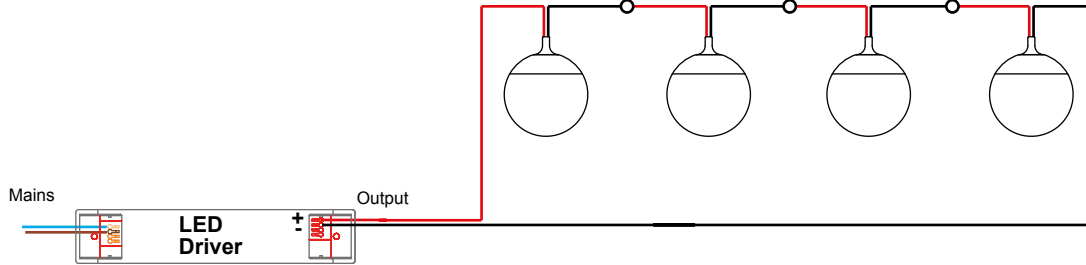
Series Wiring
