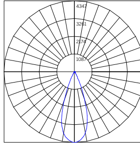
BEAM ANGLE (0-180) = 37.1° BEAM ANGLE (90-270) = 37.1°
