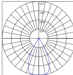
BEAM ANGLE (0-180) = 53.0° BEAM ANGLE (90-270) = 54.3°
