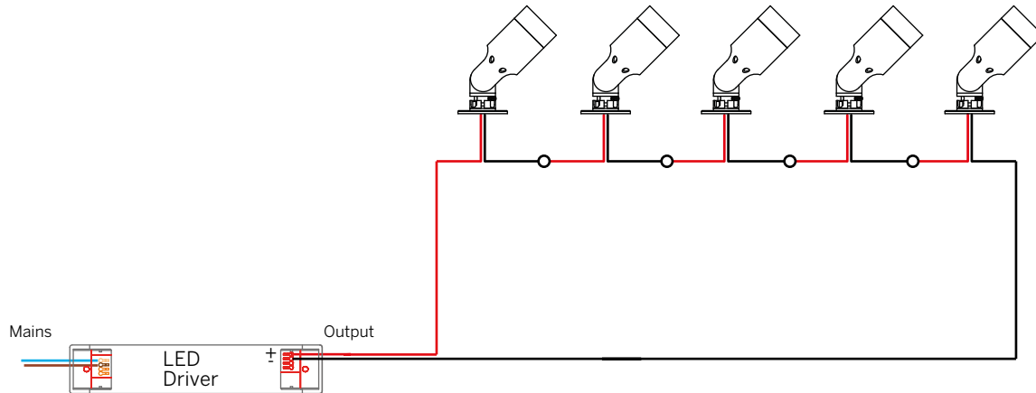
Series Wiring
