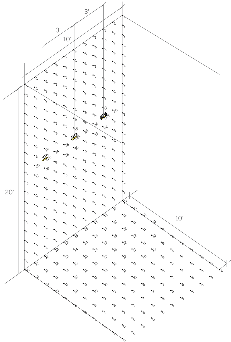
SKI-WWH-DAS-8-22-ID-30-AS 20'-0" ceiling height Floor and wall illuminance values
