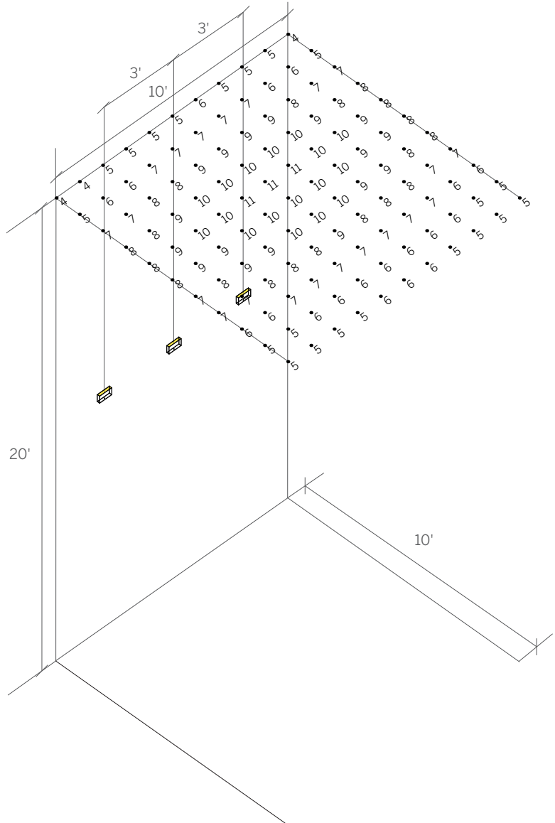
SKI-WWH-DAS-8-22-ID-30-AS 20'-0" ceiling height Ceiling illuminance values
