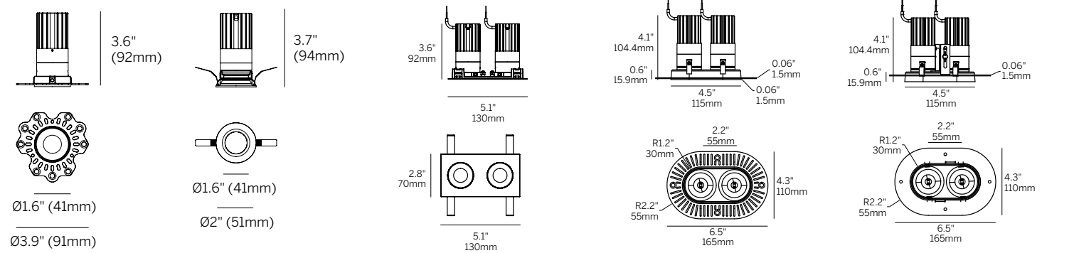
Plaster Trim (RPT) Cutout: Ø2.1" (54mm)
