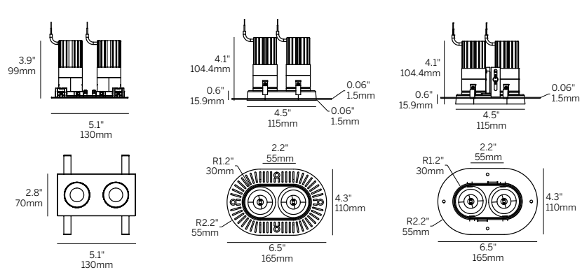
Rectangular Twin Trim with Bezel Trim (RTTBT) Cutout: 1.4" x 4.7" (60 x 120mm)
