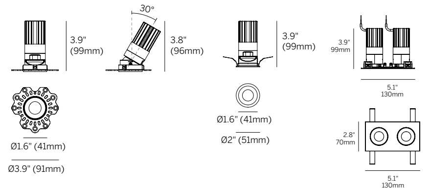
Plaster Trim (RPT) Cutout: □ 2.1" (50mm)
